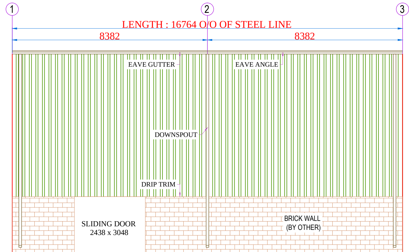
SIDE WALL SHEETING
