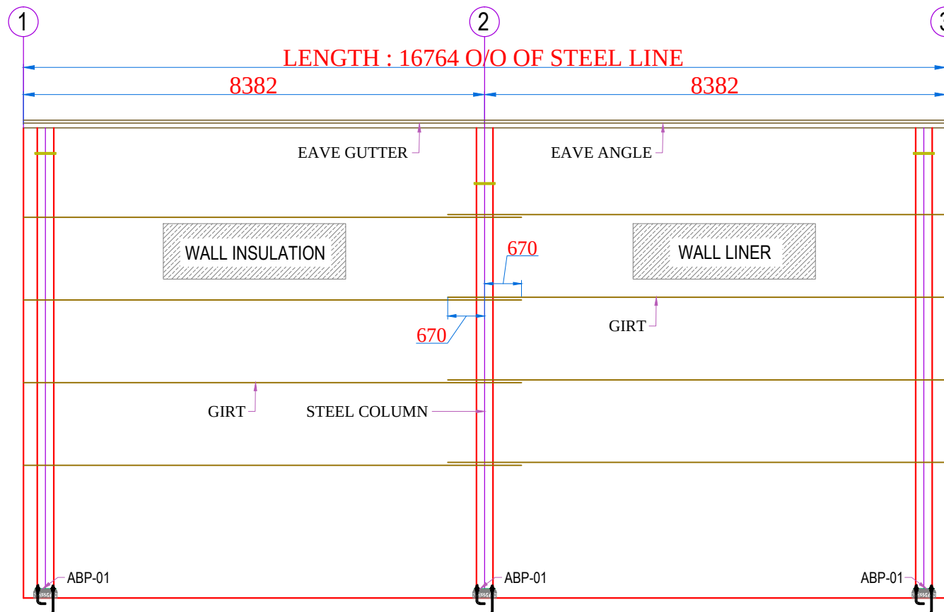
SIDE WALL FRAMING
